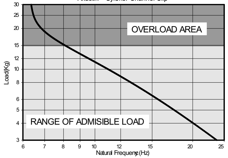
NATURAL FREQUENCY GRAPH Akustik + Sylomer Channel Clip
