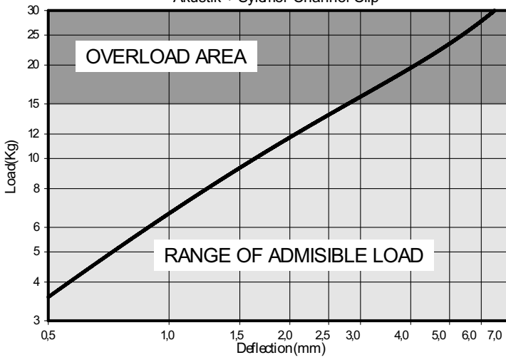
LOAD-DEFLECTION GRAPH Akustik + Sylomer Channel Clip
